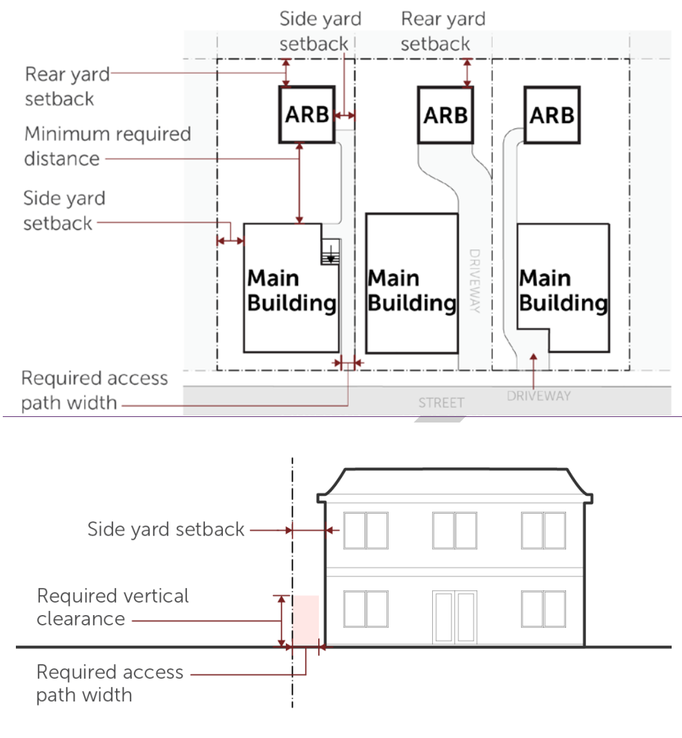
Figure 6: Section 3.18 (4) – Access Path Requirements for Additional Residential Units
