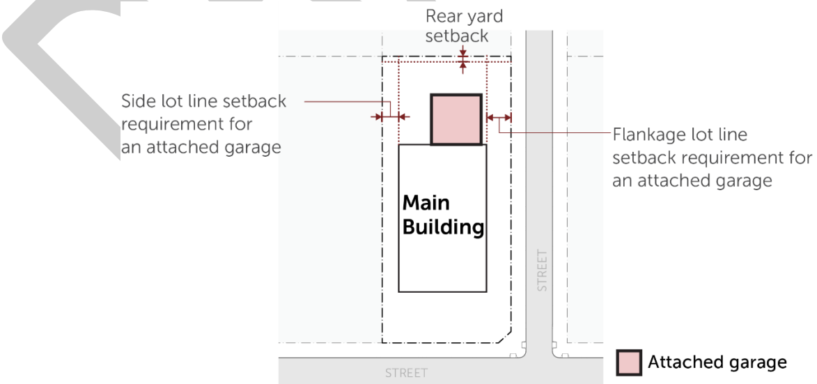
Figure 4: Section 3.13.1 – Provision for Attached Garages Located in the Rear Yard
