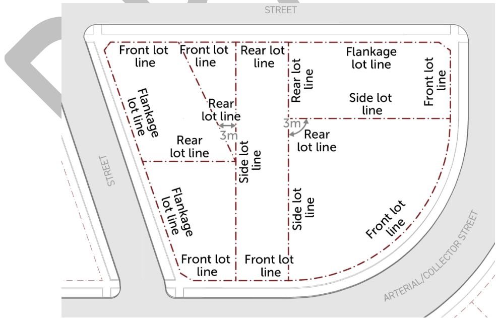
Figure 27: Section 12 – Lot Line
