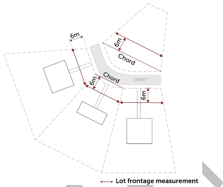
Figure 26: Section 12 – Lot Frontage
