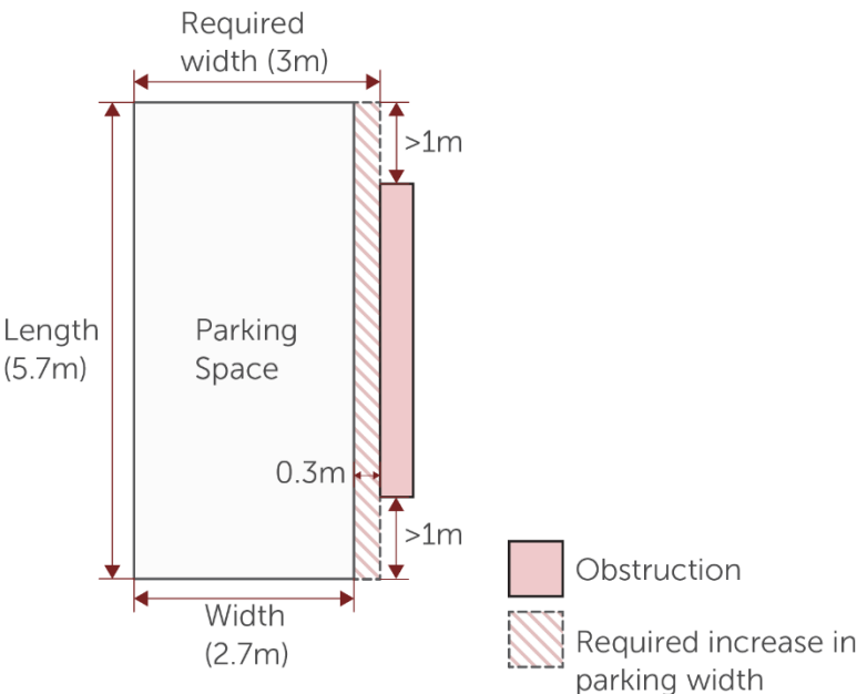
Figure 17: Section 11.6.2 – Obstruction of a Parking Space
