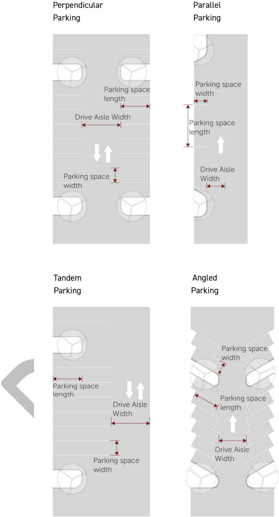
Figure 16: Section 11.6.1 – Automobile Parking Space Provisions
