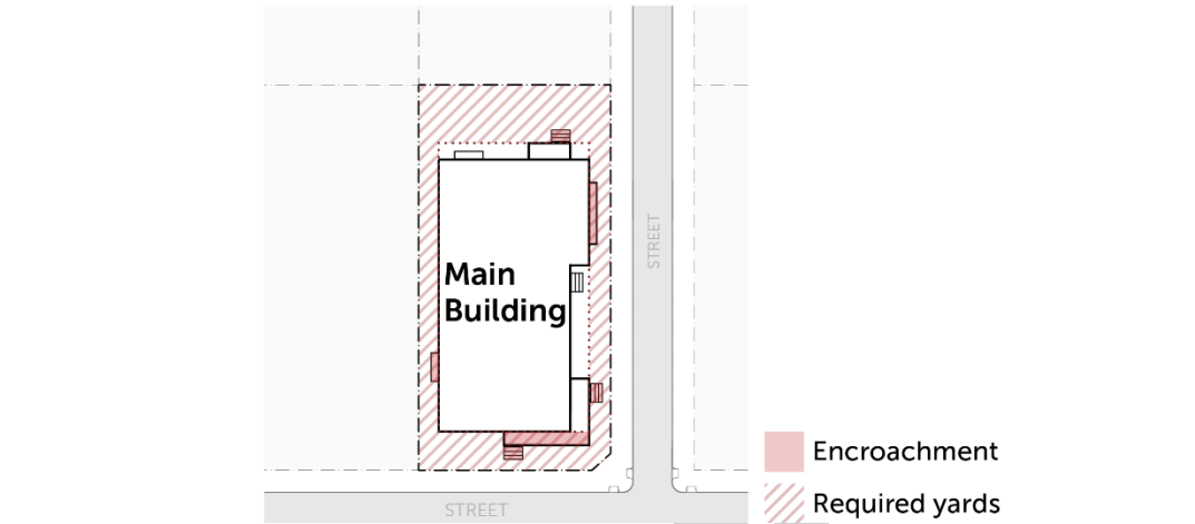
Figure 1: Section 3.4 – Permitted Encroachments into a Minimum Required Yard
