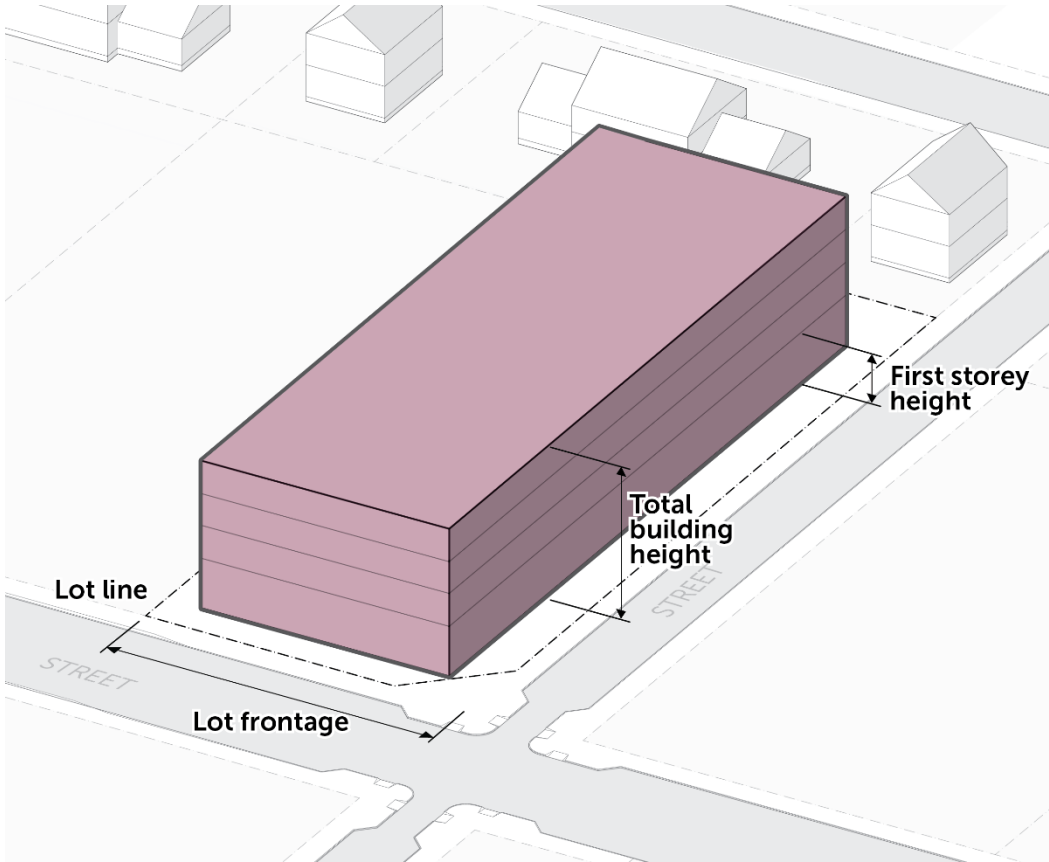
Figure 13: Table 4.2A – Low-Rise Building Standards
