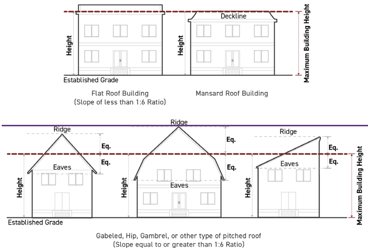
Figure 14: Section 11 — Building or Structure Height of less than 5 Storeys
