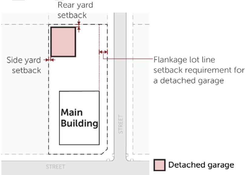
Figure 5: Section 3.13.2 – Provisions for Detached Garages
