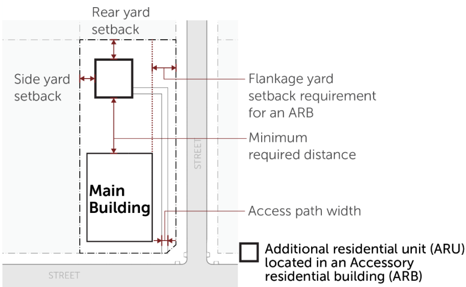
Figure 7: Section 3.18 – Additional Residential Units
